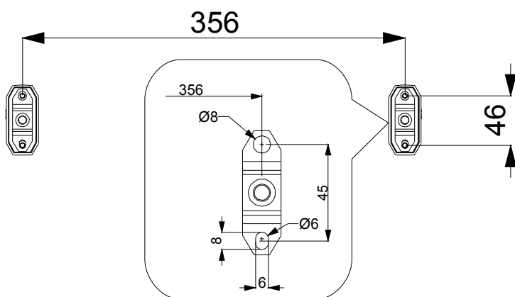
Drilling template for each arm support
